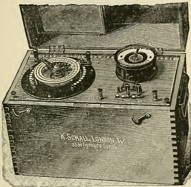
FIG. 110. — Portable battery with collector and galvanometer.
